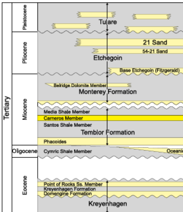
Figure 6: Sheep Springs stratigraphic section
