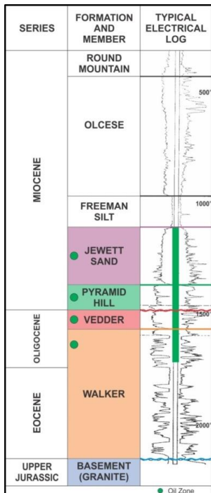
Figure 3: Round Mountain stratigraphic section
