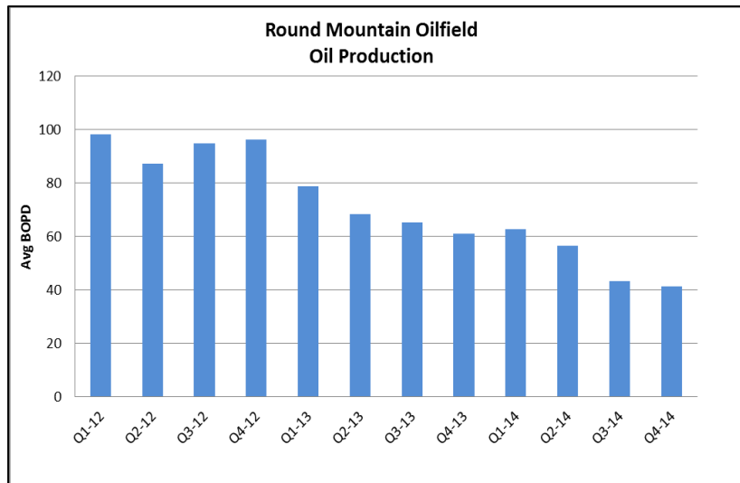
Figure 5: Round Mountain oil production 2012-14 (avg bopd)
